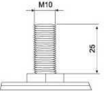
丝杆 Threaded stem
