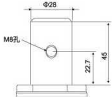
插杆(圆) Solid Stem(Round)
